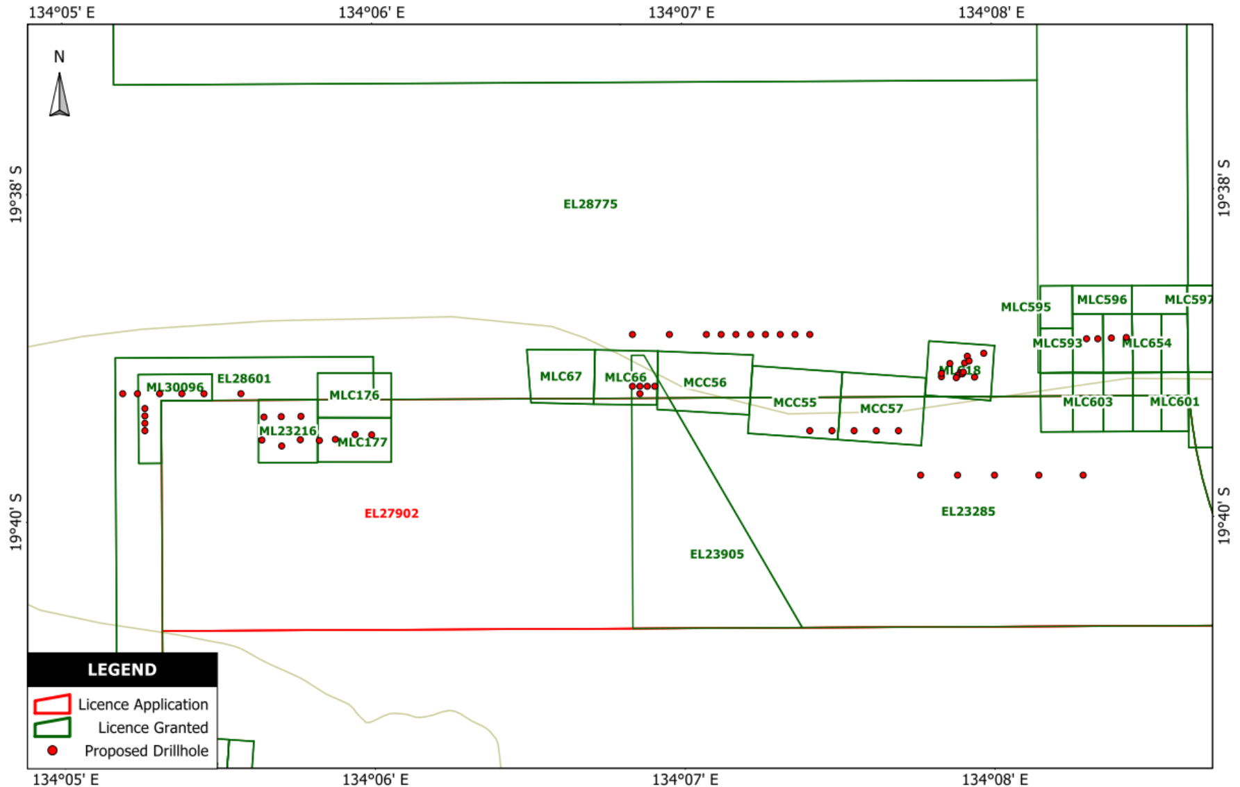
EMMERSON RESOURCES LTD 2021 PROPOSED DRILLHOLES SOUTHERN PROJECT LOCATION MAP
